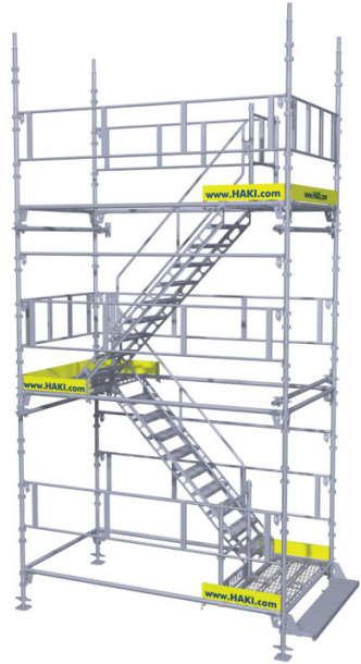
HAKI Stair Tower Symmetrical – anticlockwise ascent
