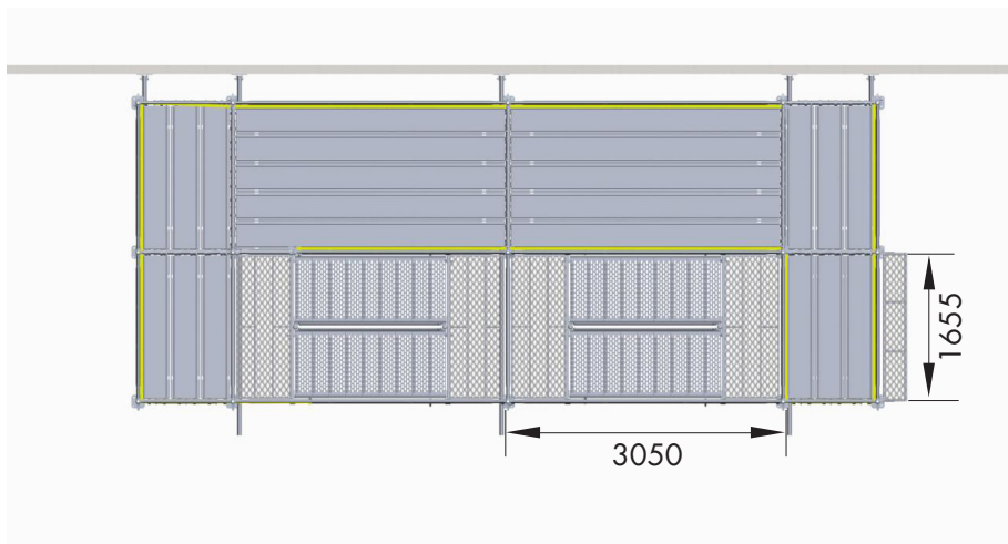
HAKI Stair Tower with double stair flights over two bays, extended landings and access via scaffold
