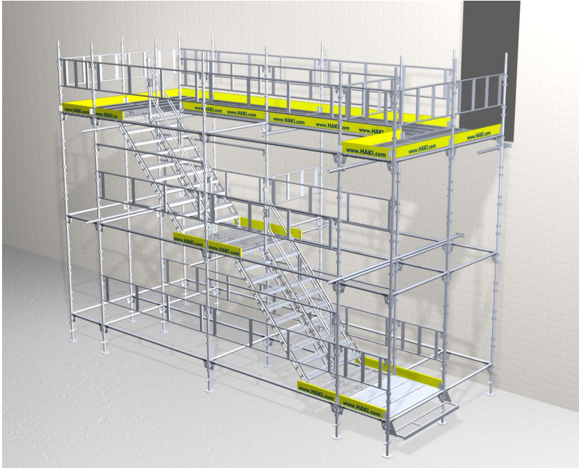
HAKI Stair Tower with double stair flights over two bays, extended landings and access via scaffold
